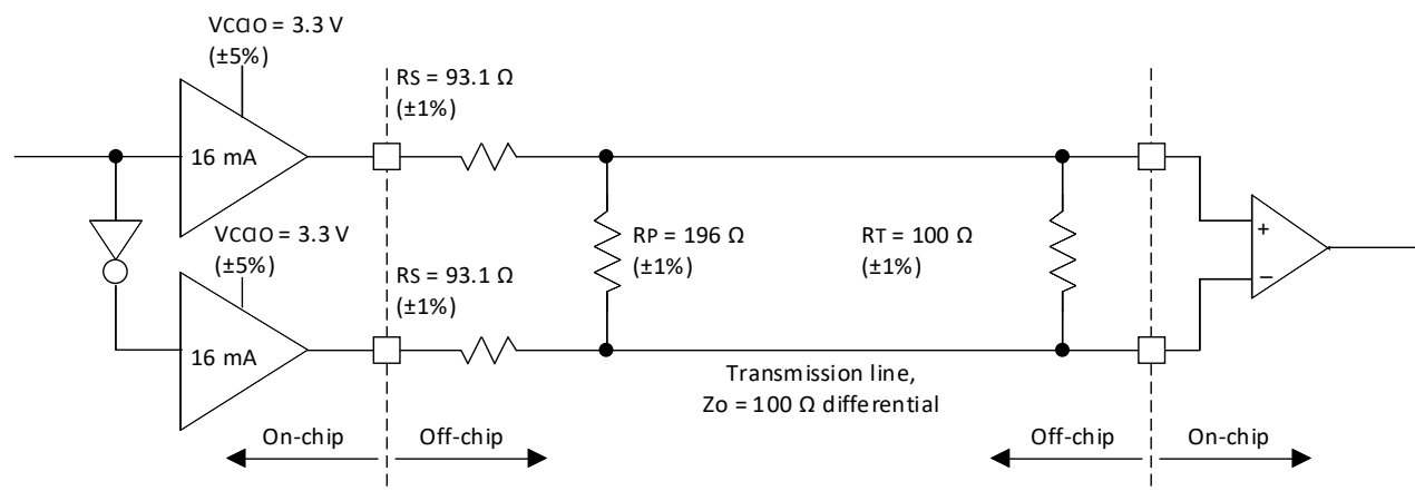
Figure 3.3. Differential LVPECL33
