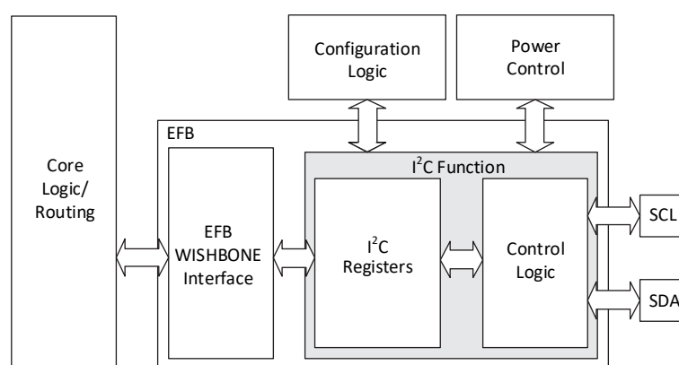
Figure 2.21. I 2 C Core Block Diagram
