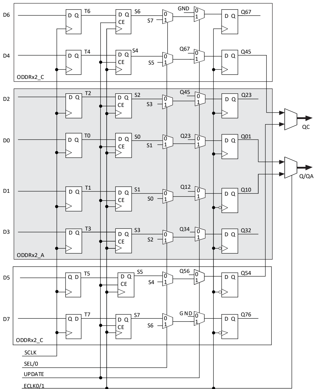
Figure 2.17. Output Gearbox
