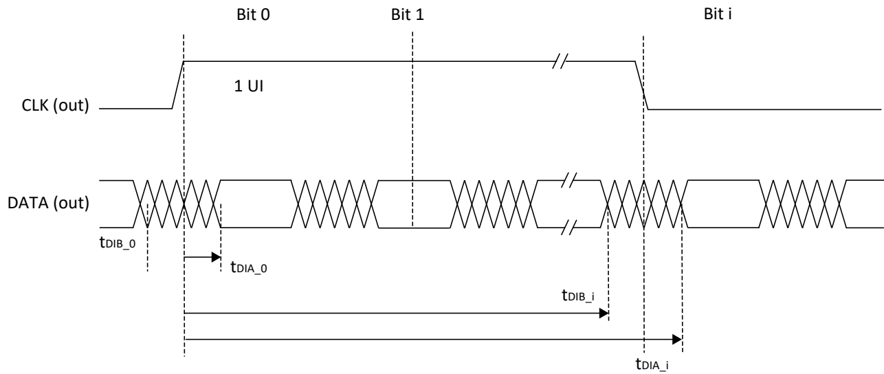
Figure 4.12. Transmitter DDRX71_TX Waveforms
